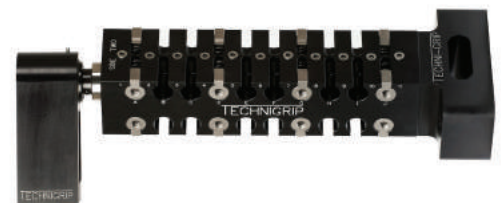
16" 4-AXIS w/ PILLOW BLOCK & PLATE PART #: MCI01-2A16-6
